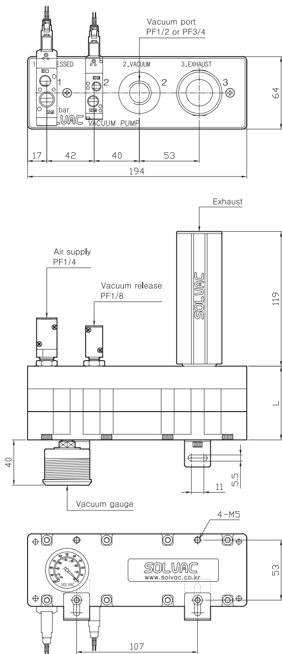
VMP/VXP type (with valve)
